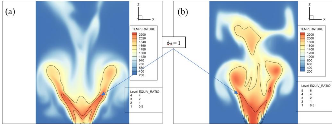
Fig. 7. 2D contour plot of the temperature for both flames: (a) Flame A and (b) Flame L, with isolines of local equivalence ratio serving to emphasize the mixture distribution concerning the flame position.
