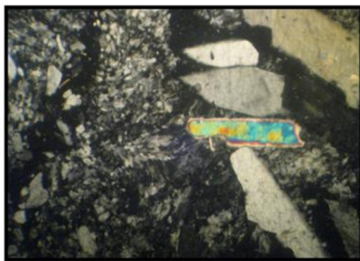
Plate 7. Anhydrite crystal , Brillion Interference colours.Duhok Dam Gypsum .X400.Crossed polars (Sample 2).
