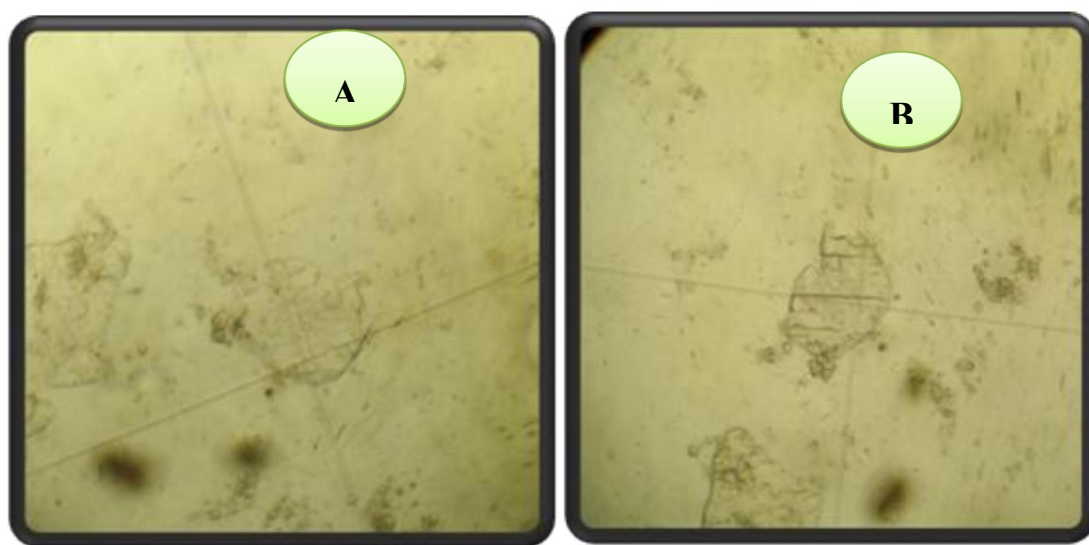
Plate 8. Dolomite crystal showing twinning. A- High Relief. B-Low Relief.X200.Crossed polars
