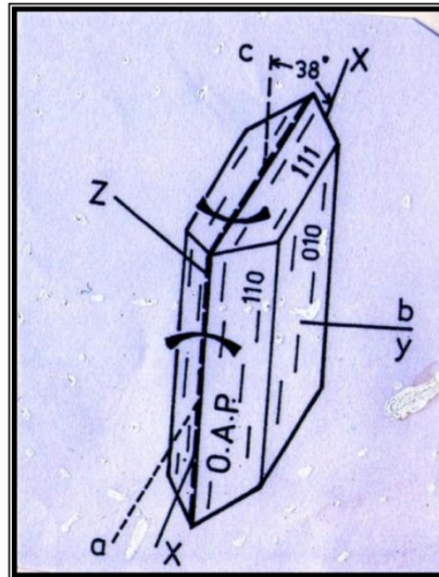
Fig. 5. Optic Orientation Diagram for Gypsum. (a, b, c) Crystallographic Axes; (X, Y, Z) Vibration Directions: (O, A, P) Optic Axial Plane. (Phillips and Griffen, 1981).
