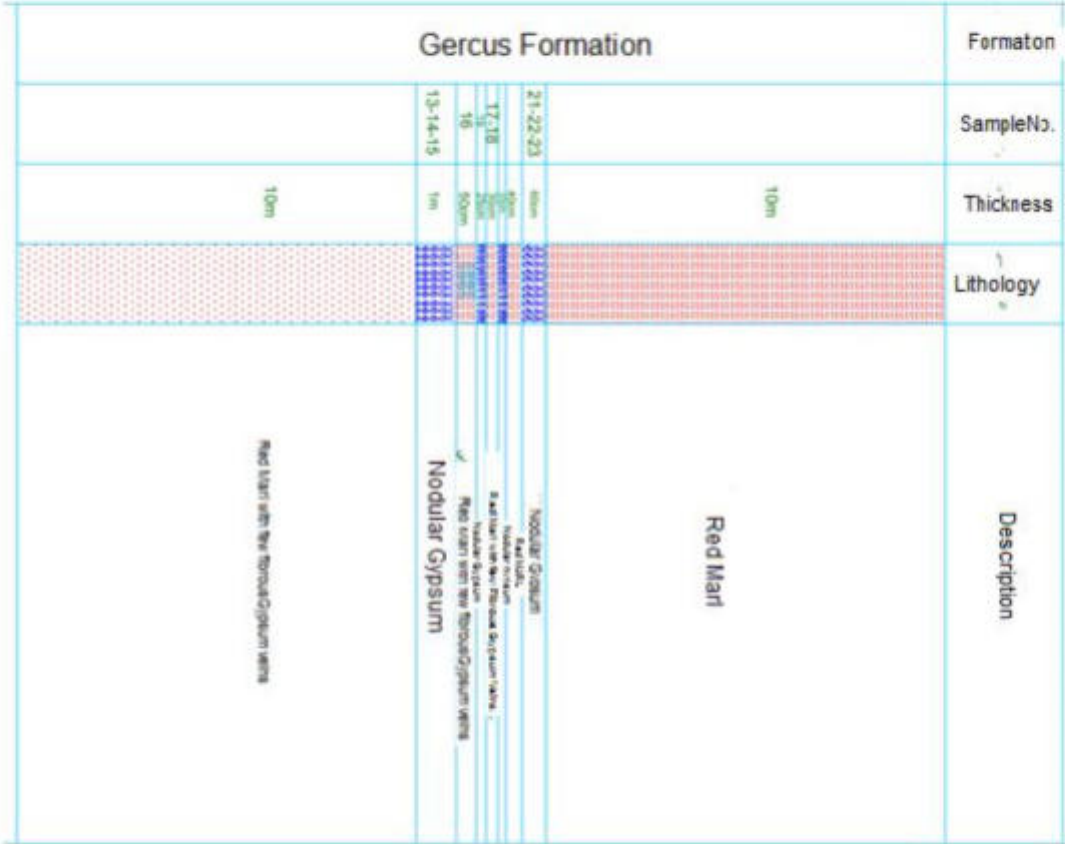
Fig. 3. Stratigraphical Section of Gypsum Gercus Formation at Zawita Junction Locality.
