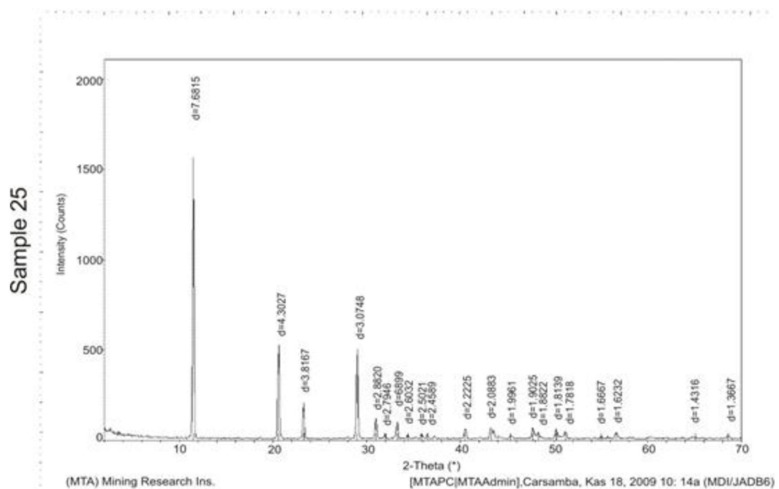
Fig.9. X-Ray Diffraction Peaks for nodular Gypsum, Baashiqia Area .Gercus Formation.
