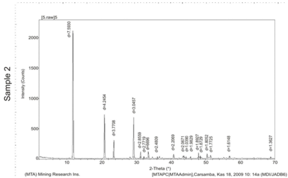
Fig. 6. X-Ray Diffraction Peaks for Massive Gypsum, Duhok Dam .Gercus Formation.
