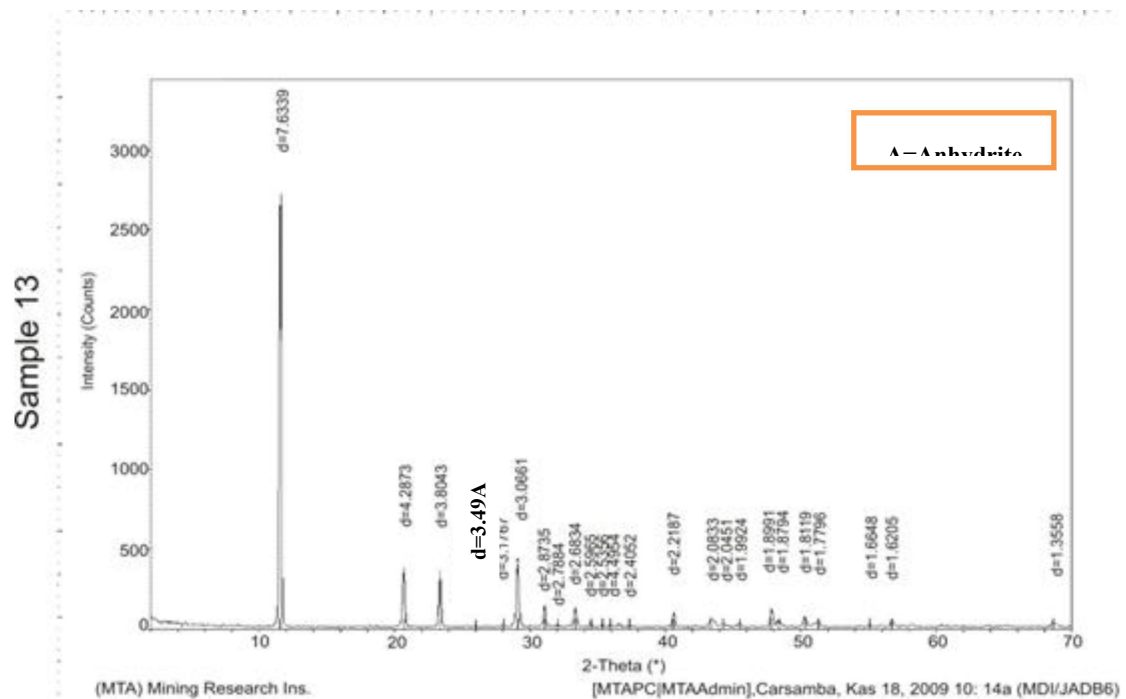
Fig. 8. X-Ray Diffraction Peaks for nodular Gypsum, Zawita Junction .Gercus Formation.
