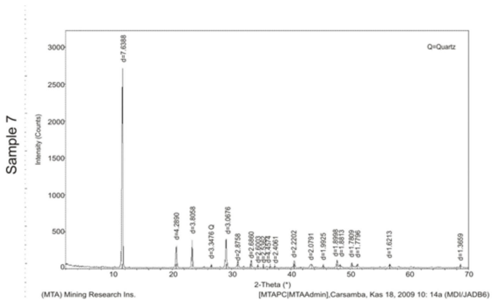
Fig. 7. X-Ray Diffraction Peaks for nodular Gypsum, Duhok Dam .Gercus Formation.
