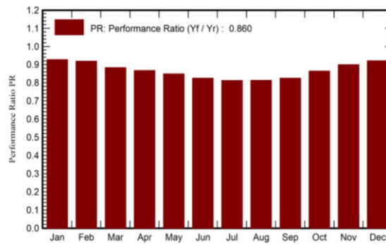
Fig. 8. Annual PR for Al_Qayarahrefinery.
